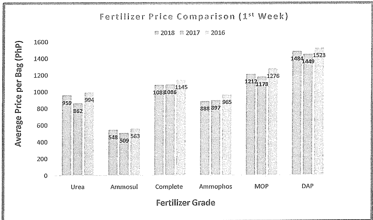
Figure 2. Three (3) year comparison of weekly fertilizer price for 6 major fertilizer grades (Week 1).
